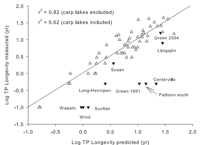
Fig. 3. Measured versus modeled treatment longevity based on TP concentrations. Filled triangles represent lakes with medium to high densities of common carp. Only the regression line for the model where carp lakes were excluded is shown.
